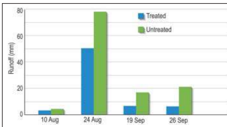
Figure 6. Daily runoff from the treated and untreated sub-watersheds in Adarsha watershed during 2000.
